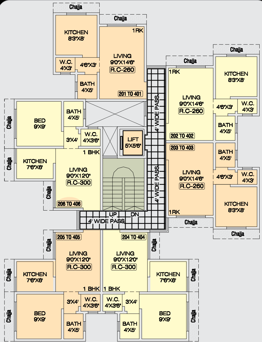
TYPICAL FLOOR PLAN (2ND TO 4TH)
